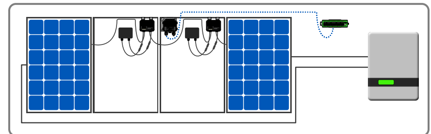
TS4-A-O, Tigo Access Point (TAP), and Cloud Connect Advanced (CCA)
