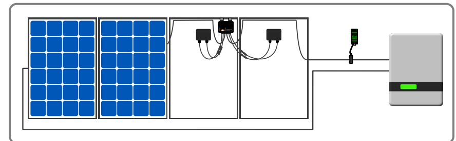
TS4-A-2F and RSS Transmitter
